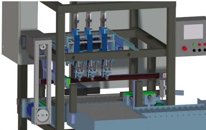
Measurement probes are used to test the plug height in relation to the surface of the lid.
