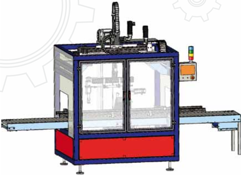
Complete, fully automatic punch press system for car and truck battery cases. Output of 5 to 6 batteries.
